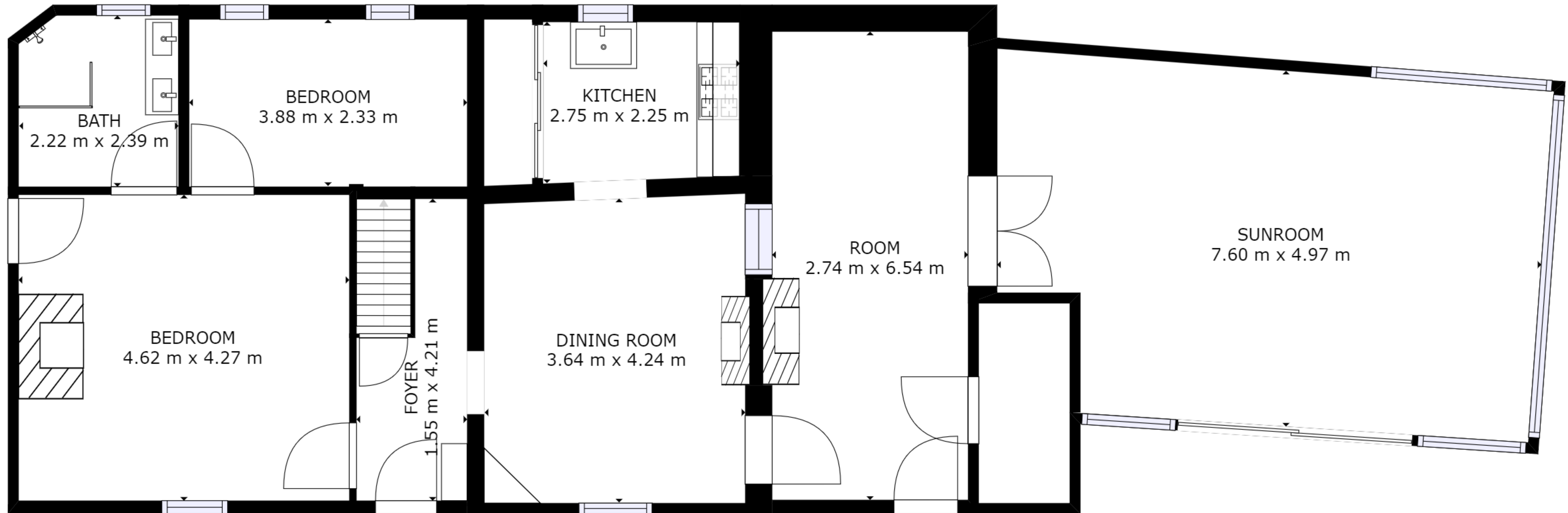
FLOOR 1
